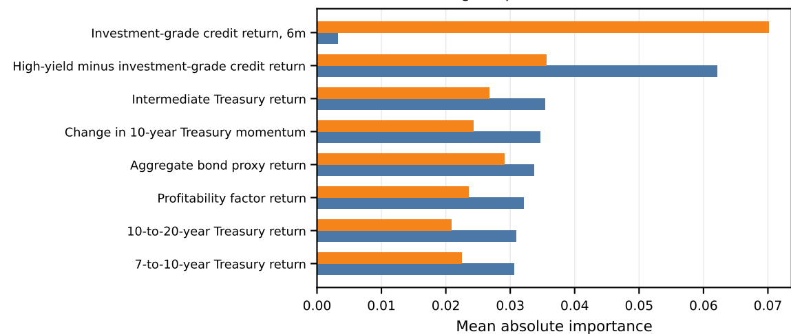
Bond regime prediction, Random forest
