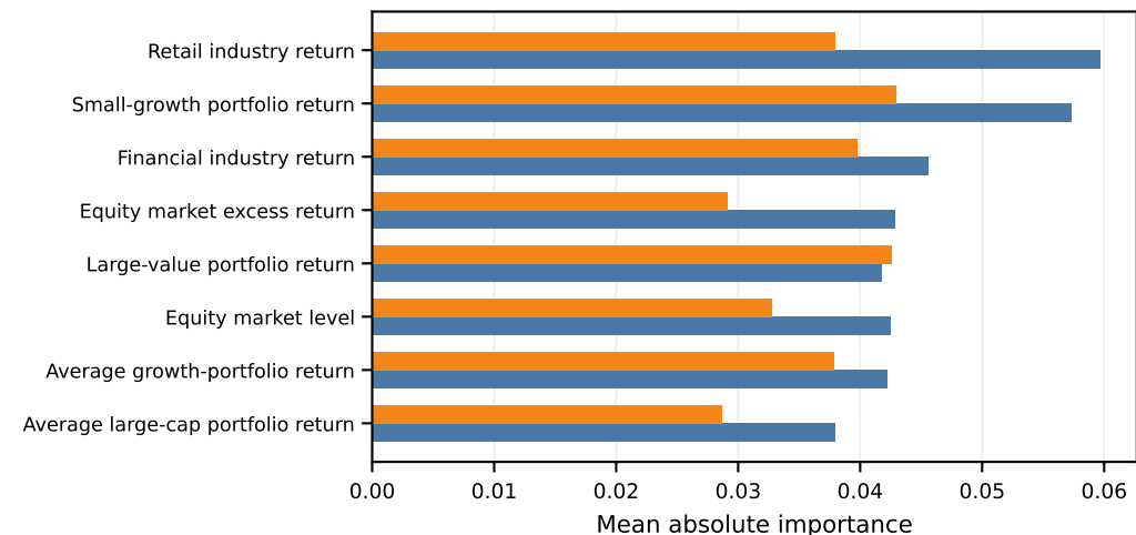
Equity regime prediction, Random forest
