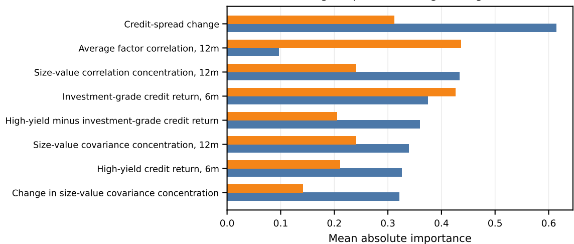
Bond regime prediction, Logistic regression
