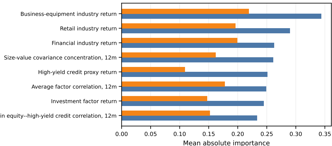
Equity regime prediction, Logistic regression
